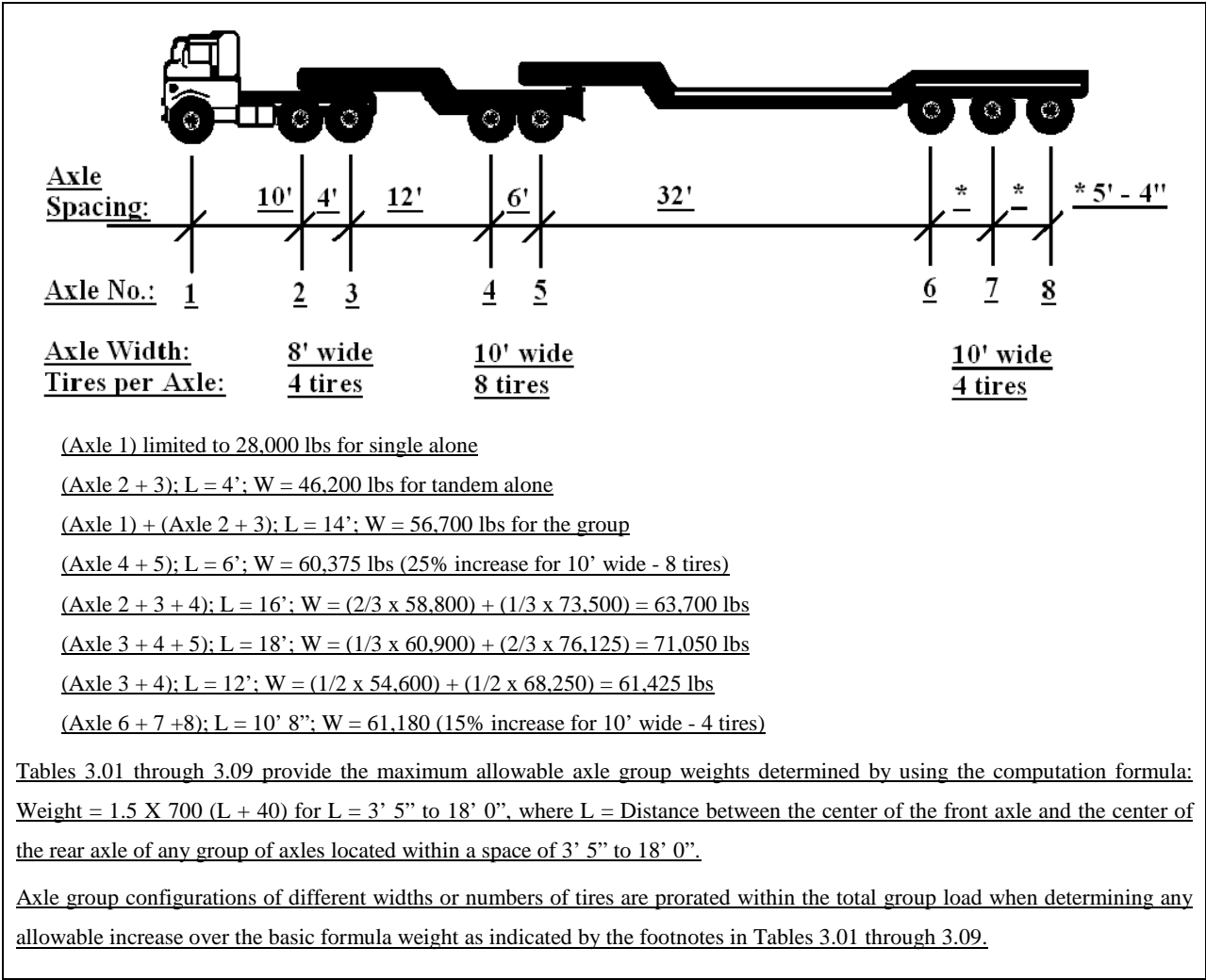
Illustration 3. Overweight Axle Group Weight Calculation
